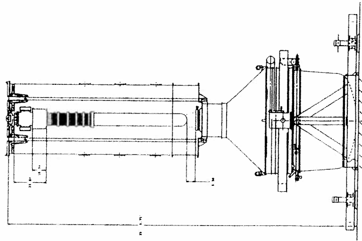
Figure 6. Probe integration with the dewar by means of an airlock and piston assembly.
