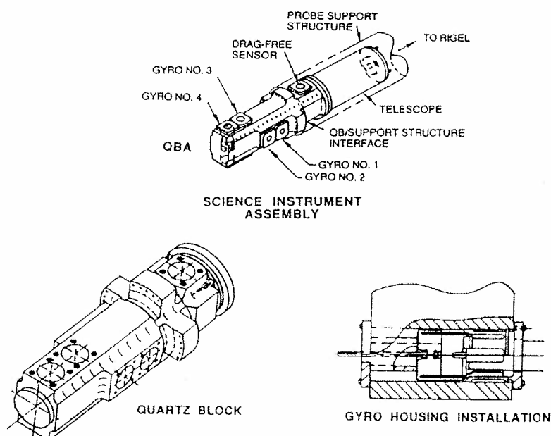
Figure 3. The Science Instrument Assembly (SIA) consists of four gyroscopes and a drag-free sensor integrated into the Quartz Block Assembly (QBA) which is optically contacted to the quartz telescope
