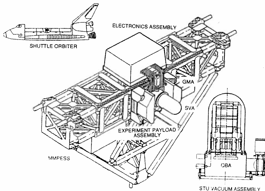
Figure 8. The Shuttle Test Unit mounted on the MPESS. This experiment will test non-cryogenic gyroscopes in low-acceleration and provides valuable experience applicable to the GP-B Science Mission.
