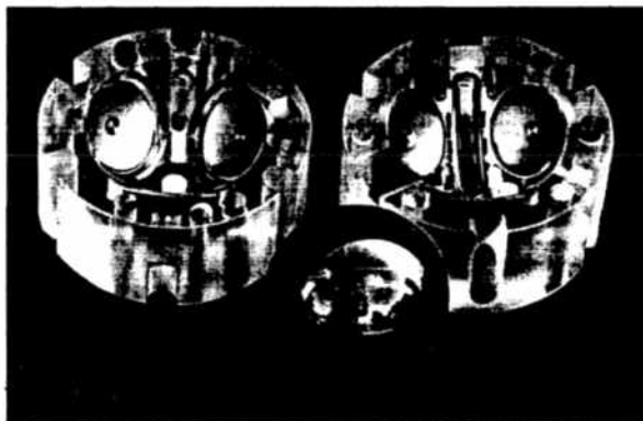
Figure 1. Photograph of a disassembled GP-B gyroscope. Shown is the quartz housing with coated electrodes (four of the six visible due to the camera angle) and coated spin-up channel. Readout loop was not yet fabricated onto this particular gyroscope's housing. Also shown is the niobium coated quartz rotor. See text for dimensions and details.
