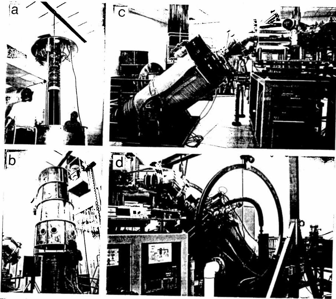
Figure 6. (a) Lowering probe in into airlock in the ~7.3 m. high Integrated Systems Tests facility. (b) Lowering airlock with probe onto dewar. (c) Dewar tilted parallel to Earth's spin axis (to minimize gyro drift due to Earth rotation) and coupled to vacuum pumps. Black boxes are suspension electronics. (d) FIST set-up during measurement of ac shielding factor. Coils of large electro-magnet straddle dewar.
