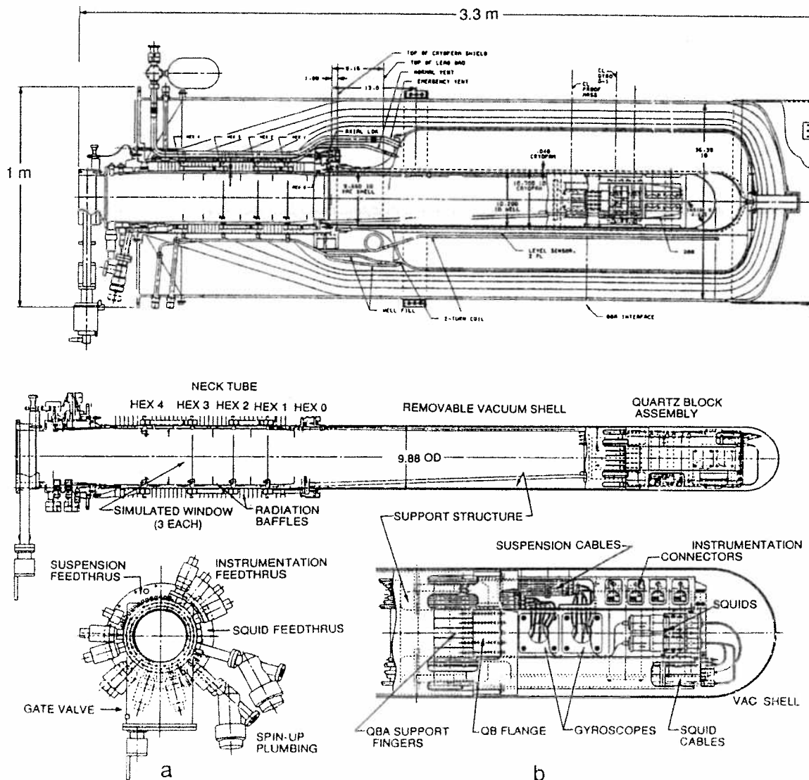
Figure 4. FIST instrument hardware. The top drawing shows the final package with the probe integrated into the EDD. In the lower drawing the probe is shown separately for greater clarity and includes views of [a] the Top Hat with its feedthroughs and gate valve, and [b] a blow-up of the SIA (QBA) region.
